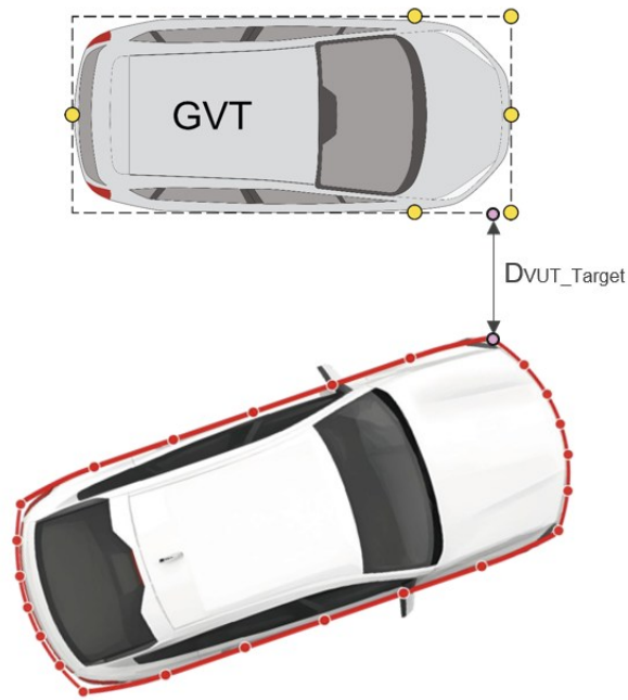
Figure 8. Closest distance illustrated in a Car-to-Car overtaking scenario
