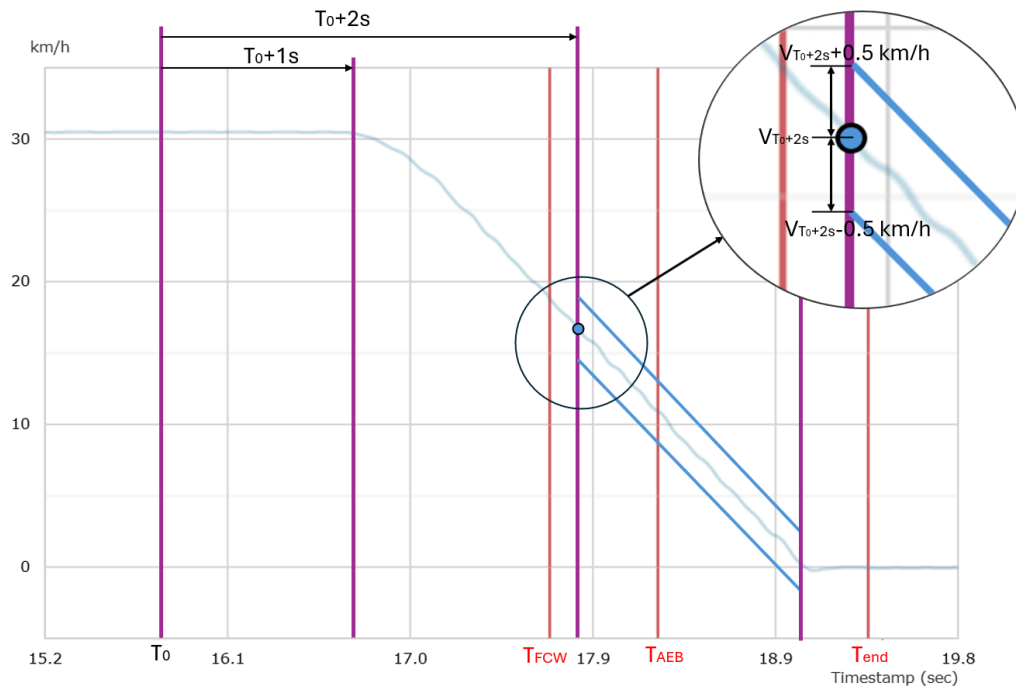
Figure 7. CMRb and CCRb target brake profile monitoring
