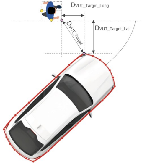
Figure 5. Illustration of the TTT calculation for a turning scenario
