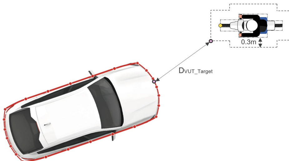
Figure 9. Closest distance illustrated in a Car-to-Motorcycle oncoming scenario
