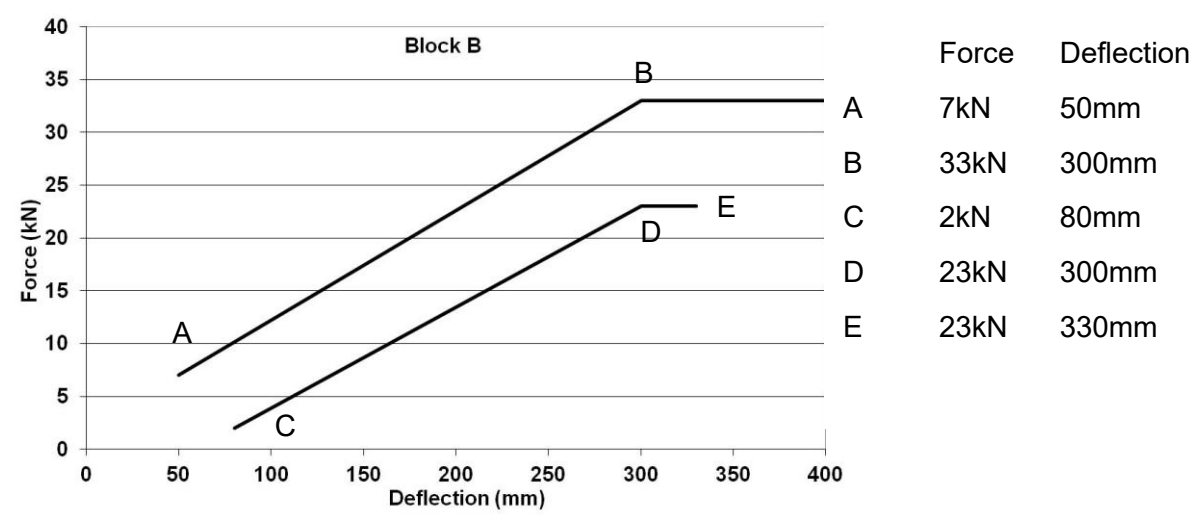
Figure 15: Block B dynamic corridor
