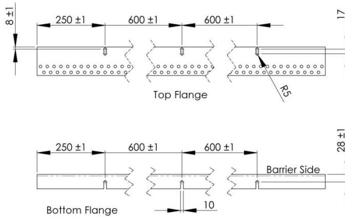
Figure 8: Top and bottom AE-MDB mounting flanges
