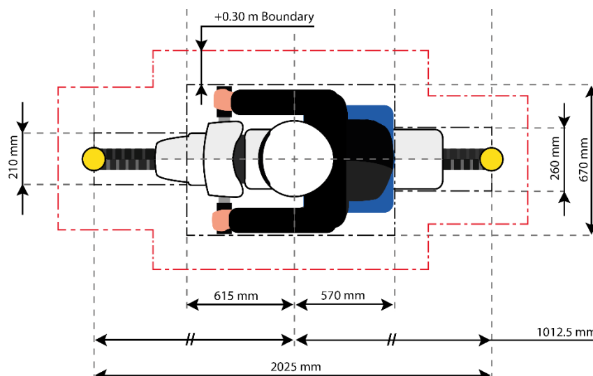
Figure 5-2: Adjusted PTW virtual box for Car-to-Motorcyclist Oncoming and Overtaking tests
