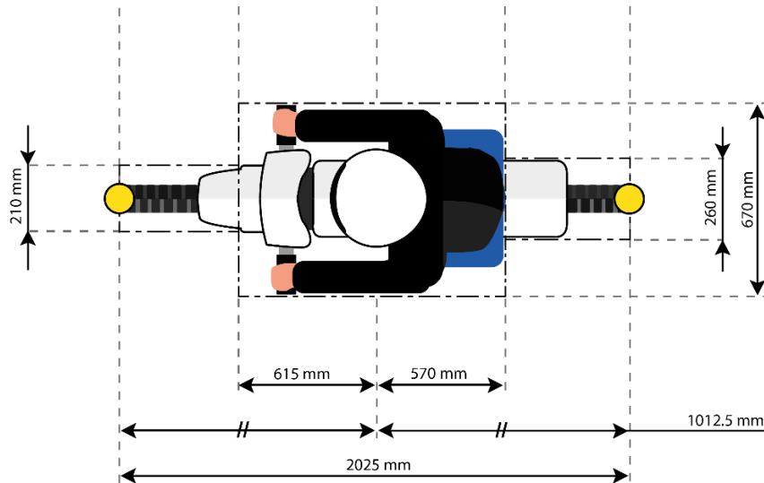
Figure 1-8 Virtual box dimensions around EMT
