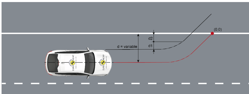
Figure 1-2 Global Coordinate System origin
