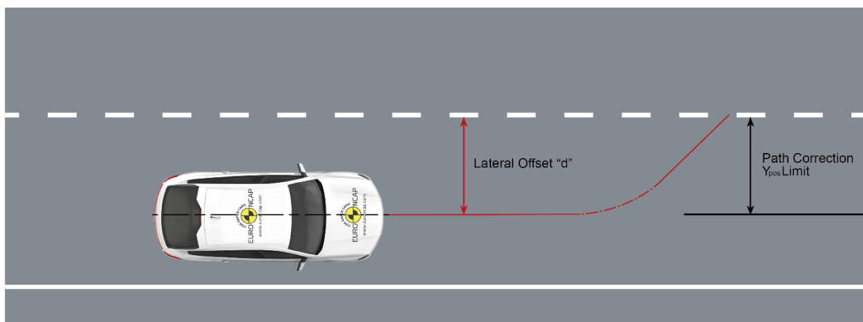
Figure 5-1: Correction Path lateral offset "d" Y_{\text{pos}} definition
