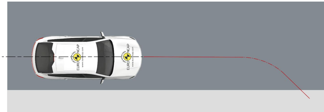
Figure 3-2 Lane Departure – ELK Road Edge test format
