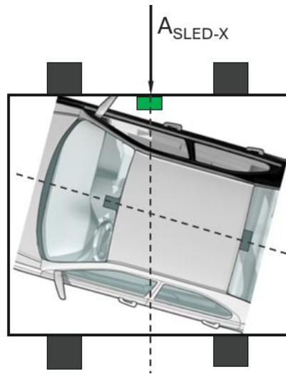
Figure 7: Sled pulse scaling
