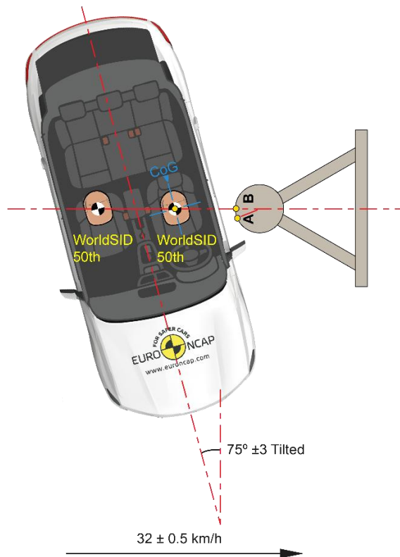
Figure 3: Pole impact location
