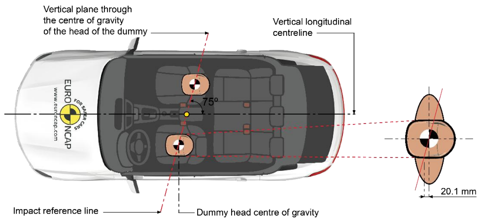
Figure 2: Pole impact reference line (IRL)
