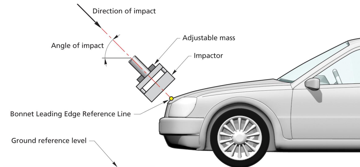
Figure 29: Upper Legform to Bonnet Leading Edge Test
