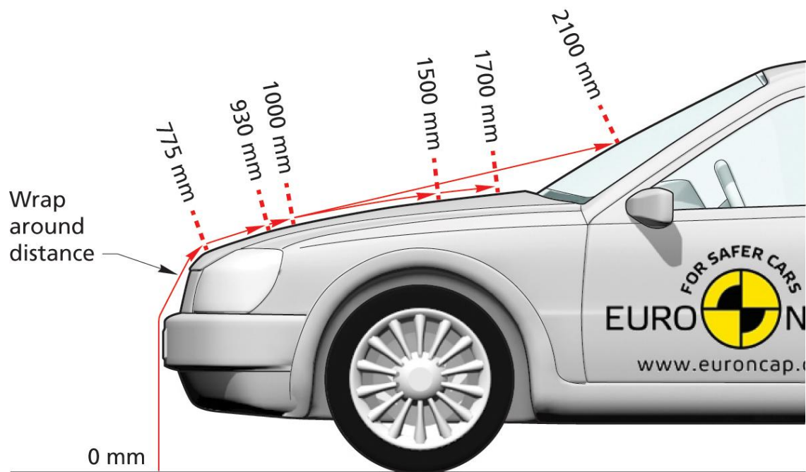
Figure 12: Marking wrap around lines
