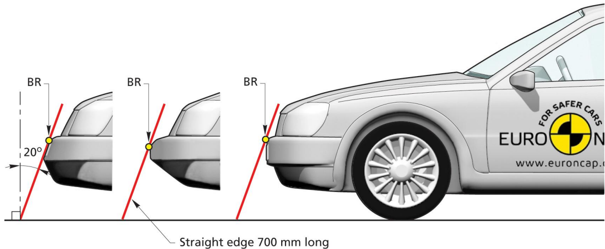
Figure 4: Determination of upper bumper reference line
