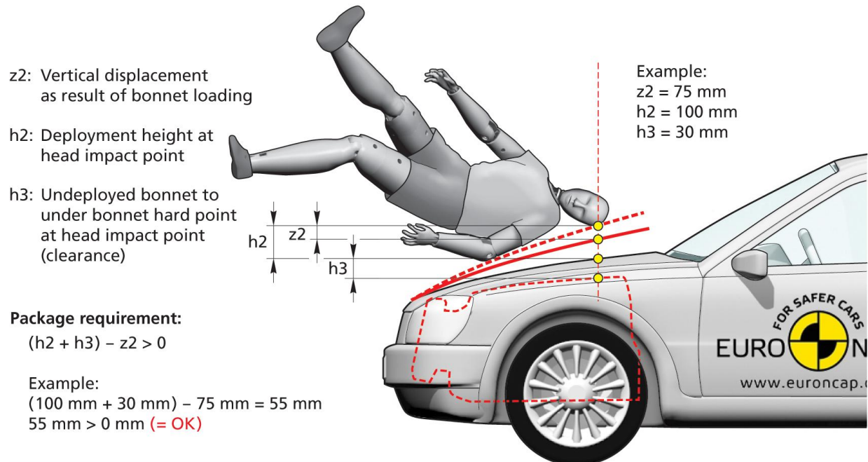
Figure 3: Bonnet deflection total clearance requirement
