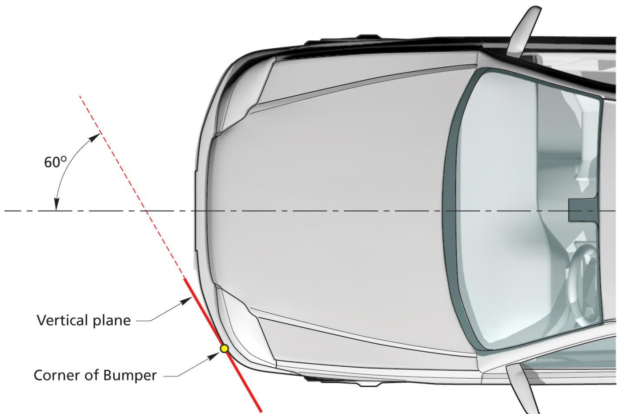
Figure 6: Determination of bumper corner
