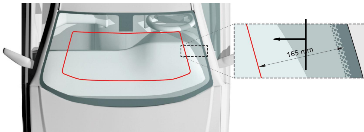
Figure 20: Windscreen periphery measurement
