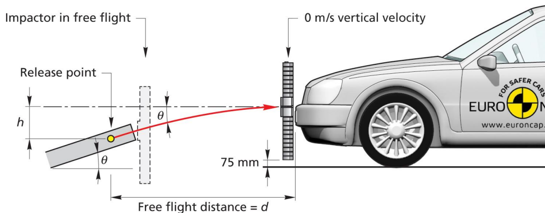
Figure 25: Ballistic Correction Procedure
