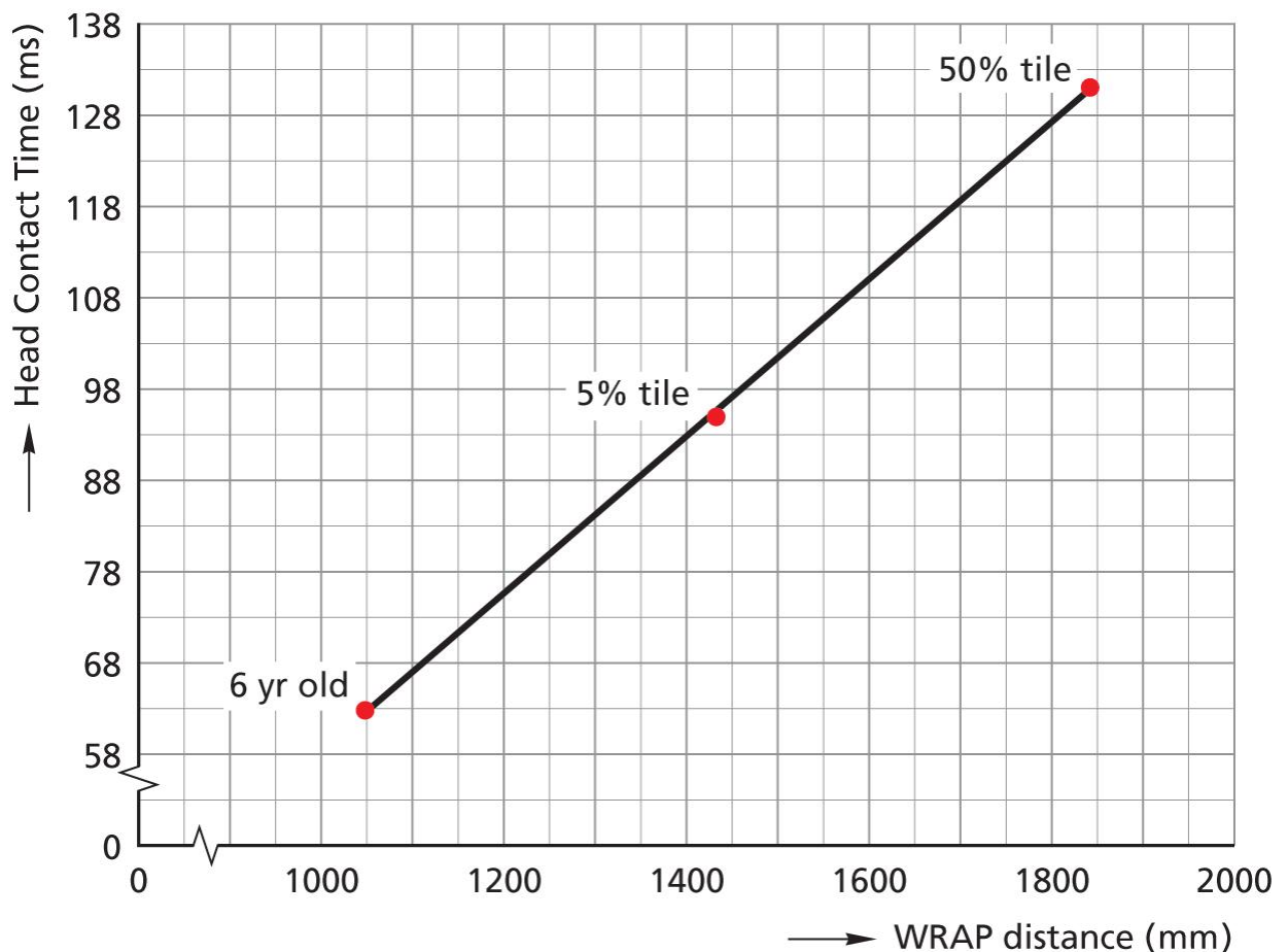
Figure 22: WAD vs HIT
