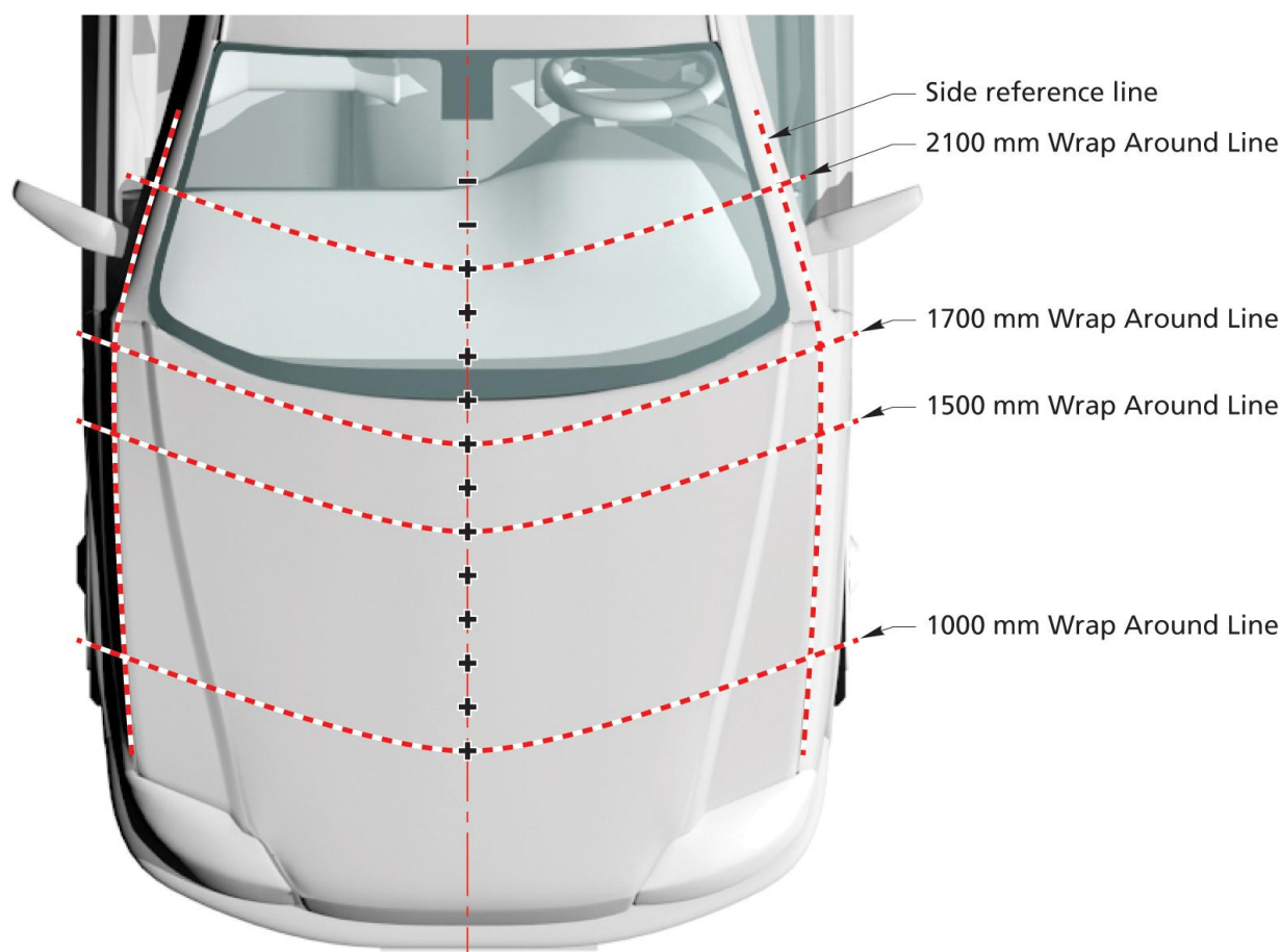
Figure 13: Headform test area
