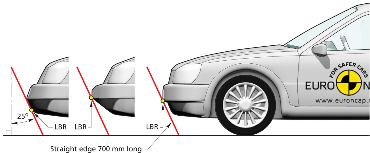
Figure 5: Determination of the Lower Bumper Reference Line
