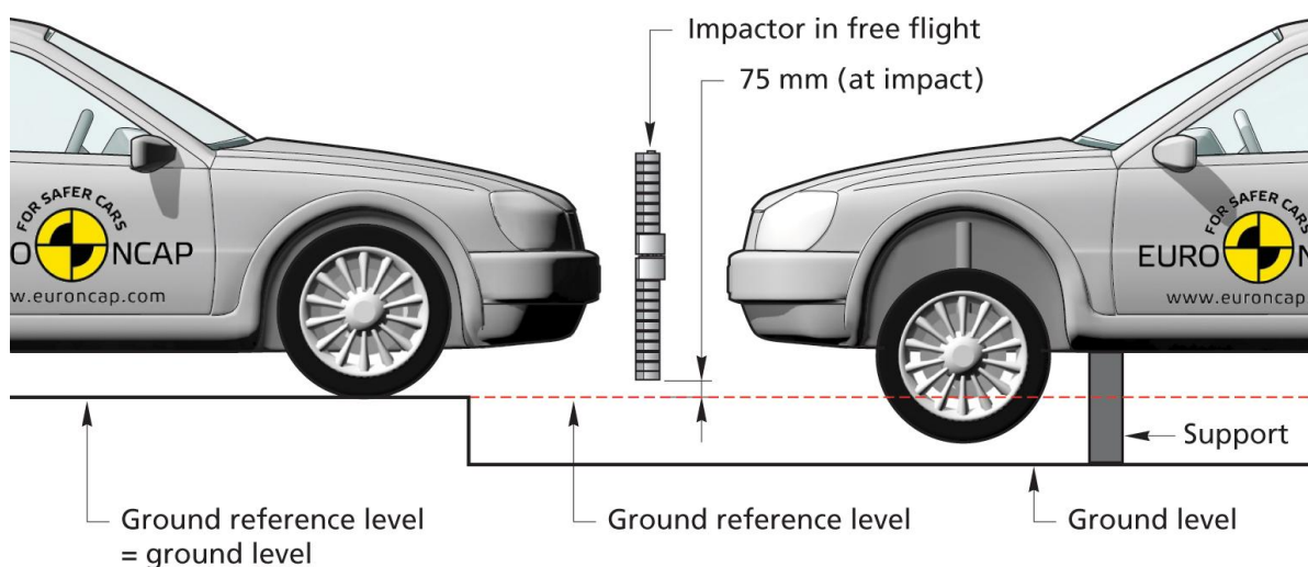
Figure 23: Legform to Bumper tests
