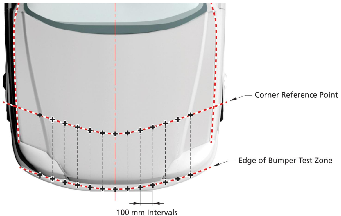
Figure 18: Division of the bonnet leading edge and upper bumper reference lines
