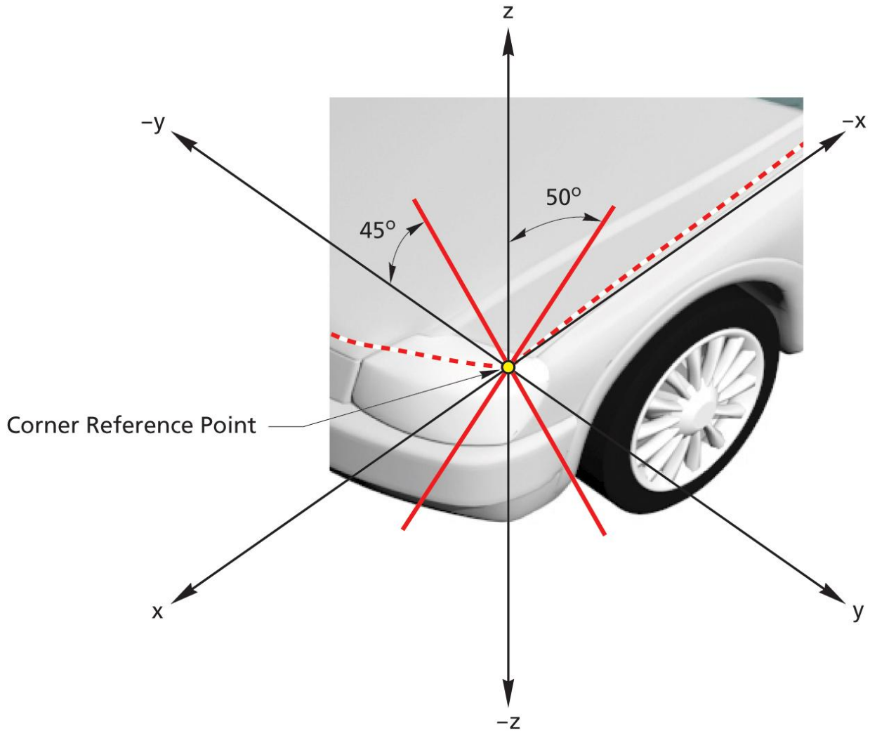
Figure 9: Determination of the corner reference point
