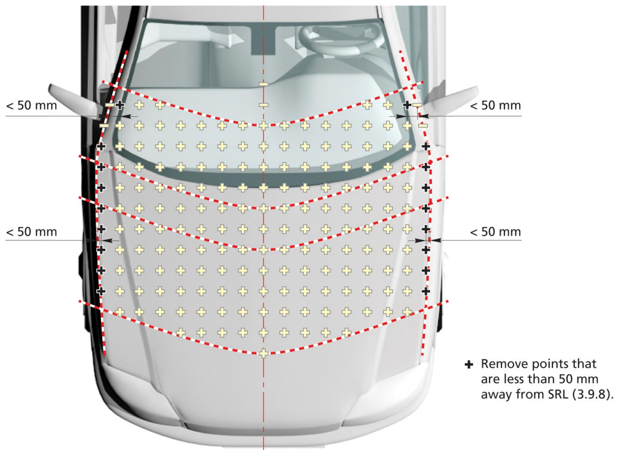
Figure 16: Deleting grid points
