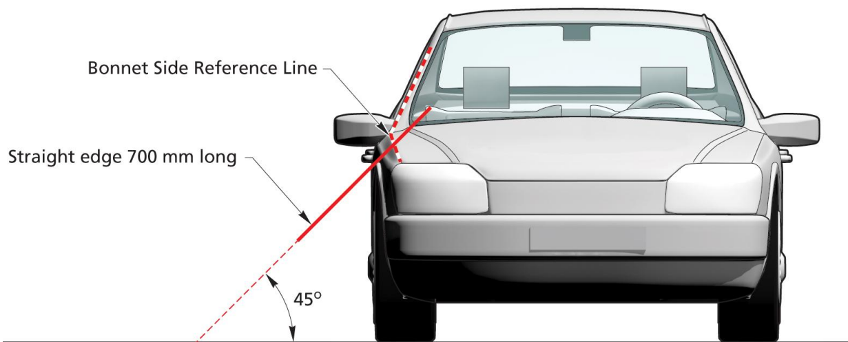
Figure 8: Determination of the bonnet side reference lines
