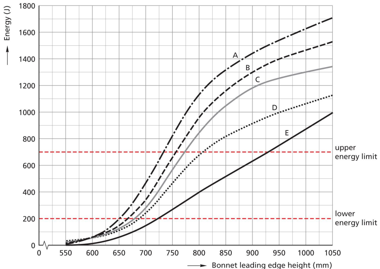
Figure 28: Kinetic energy of upper legform to Bonnet Leading Edge tests with respect to vehicle shape
