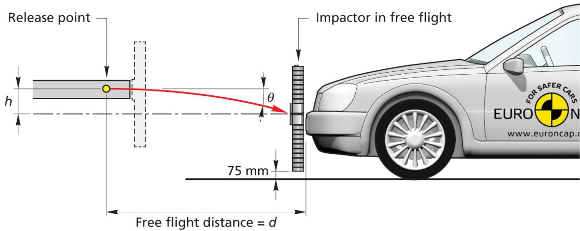
Figure 24: Droop Compensation
