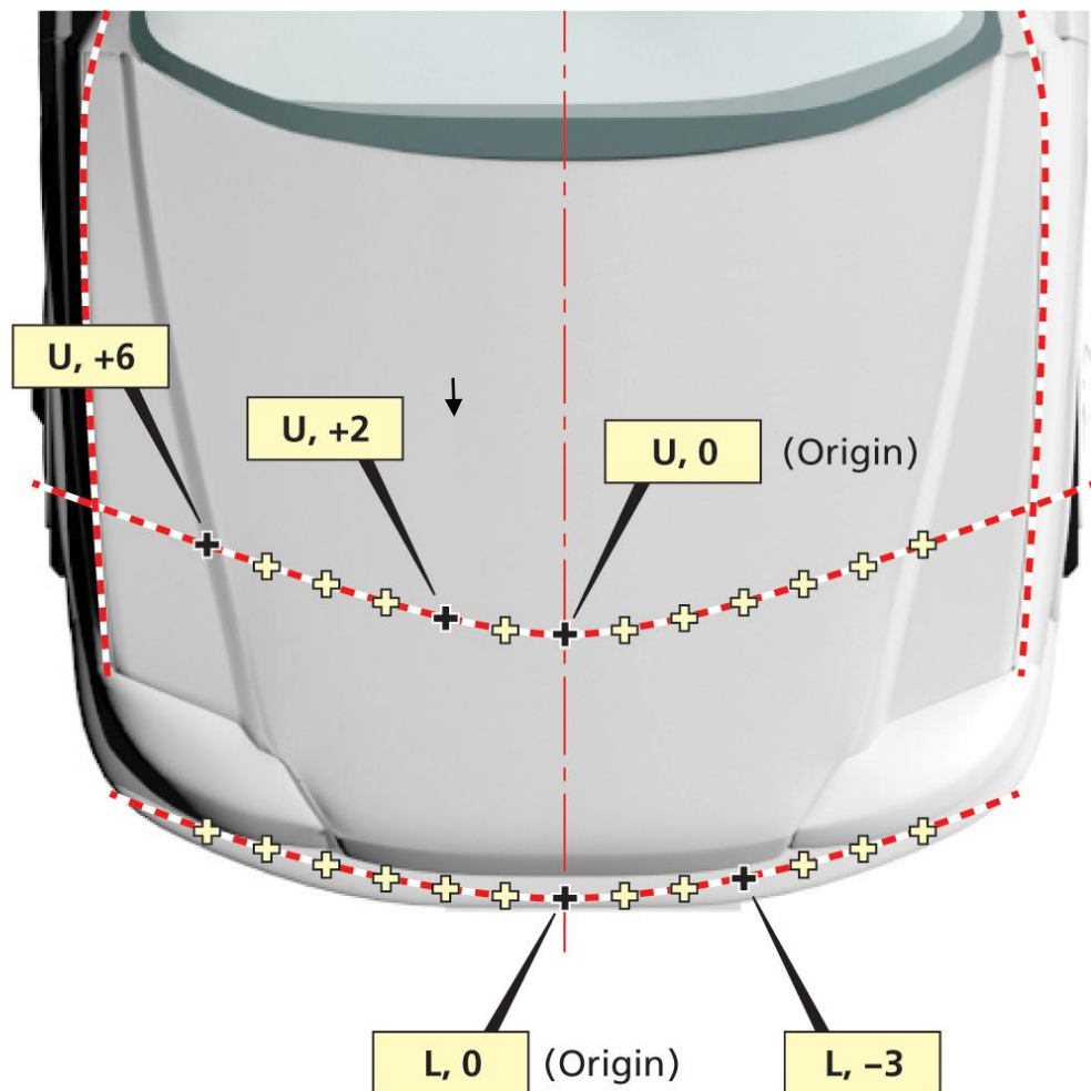
Figure 19: Labelling the bonnet leading edge and bumper test zones
