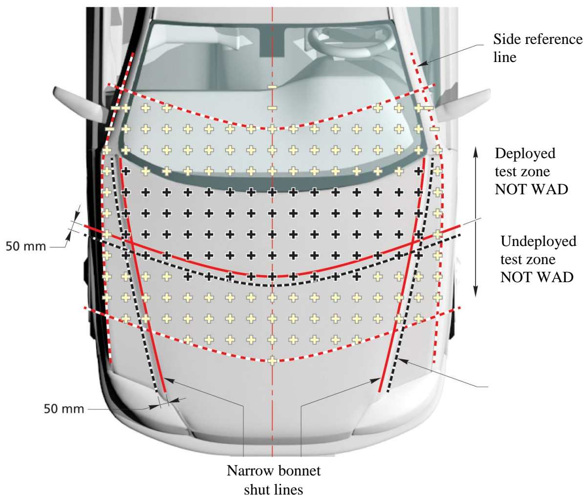
Figure 1: Area to meet low speed requirements
