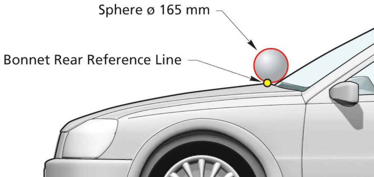
Figure 10: Determination of the bonnet rear reference line
