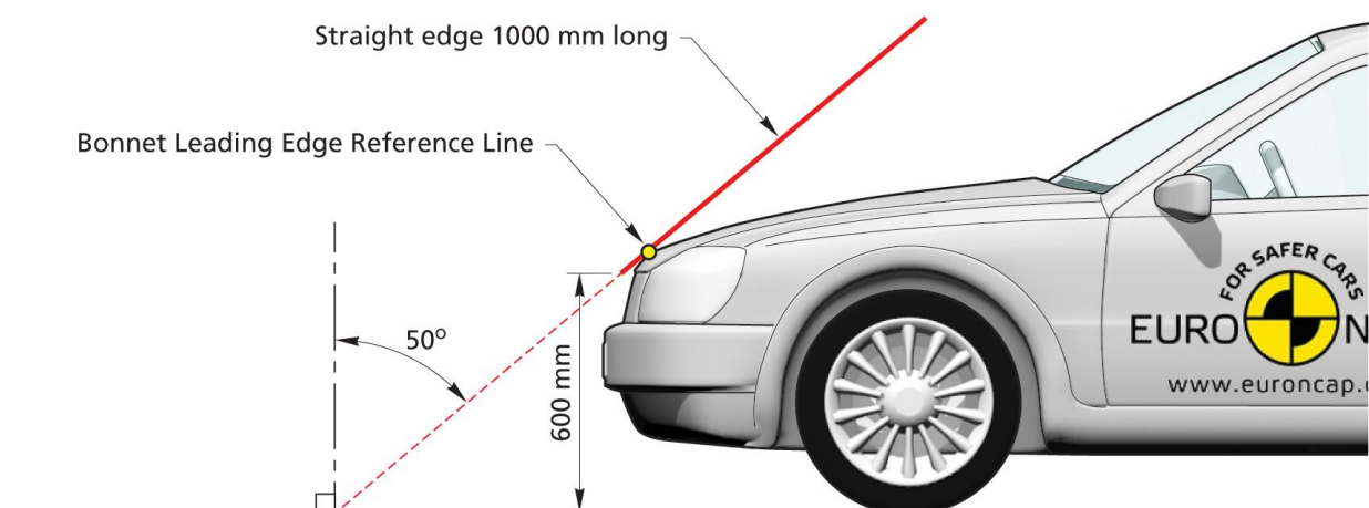
Figure 7: Determination of the Bonnet Leading Edge Reference Line
