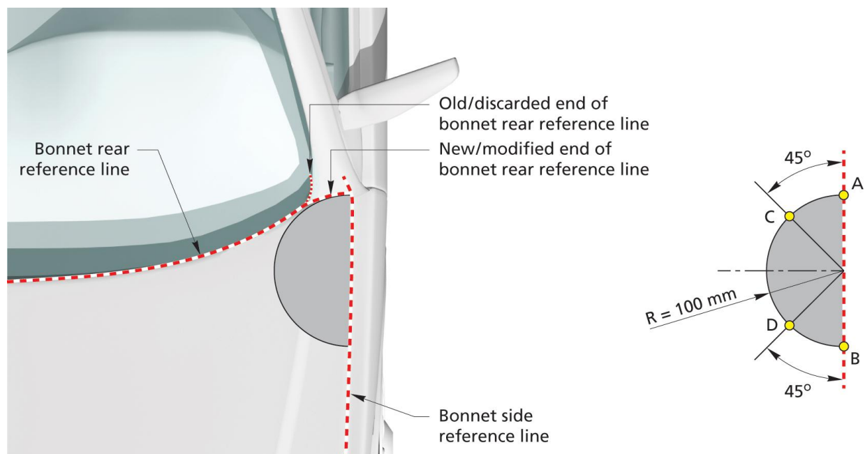
Figure 11: Bonnet rear reference line template and extension
