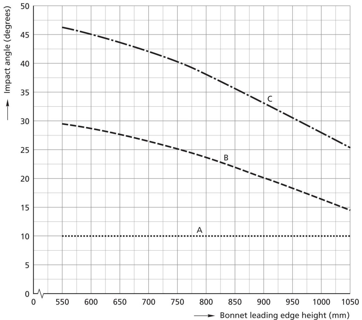
Figure 27: Angle of upper legform to Bonnet Leading Edge tests with respect to vehicle shape
