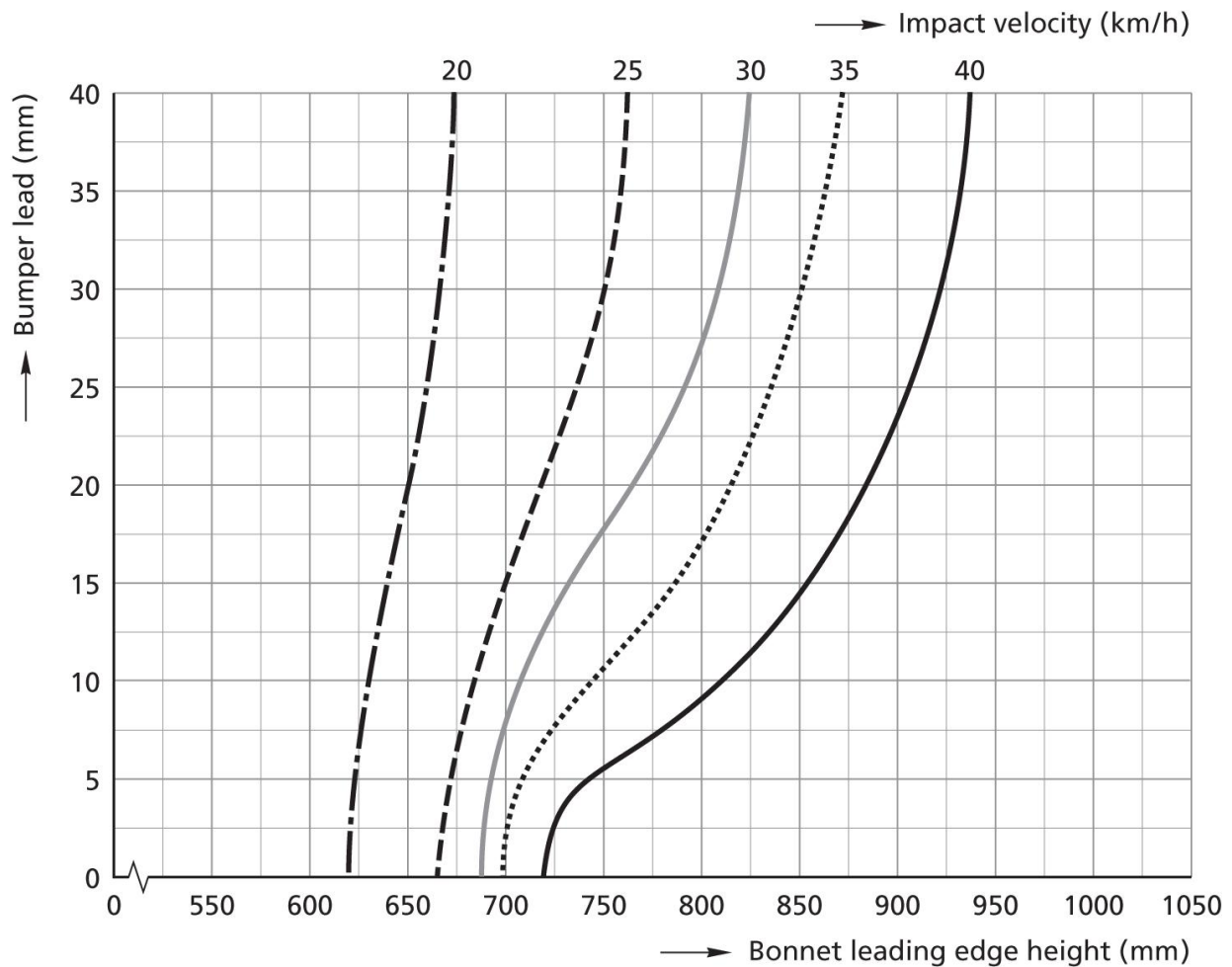
Figure 26: Velocity of upper legform to Bonnet Leading Edge tests with respect to vehicle shape
