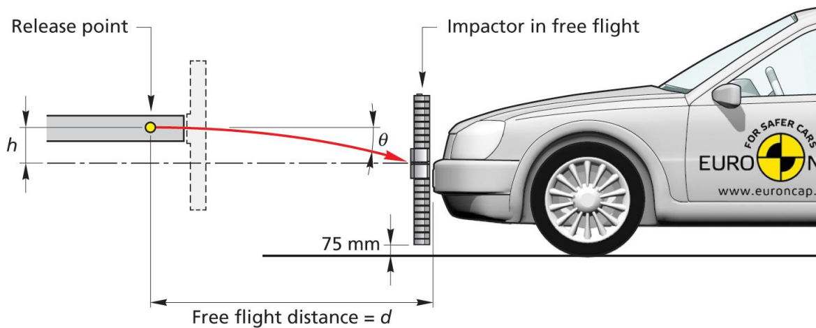
Figure 26: Droop Compensation
