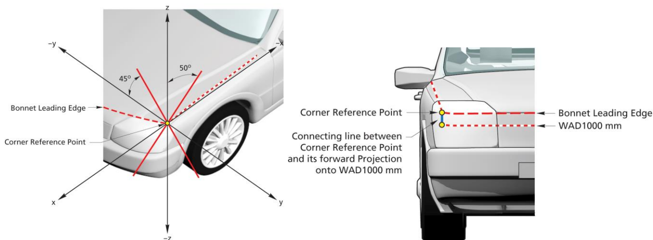
Figure 10: Determination of the corner reference point
