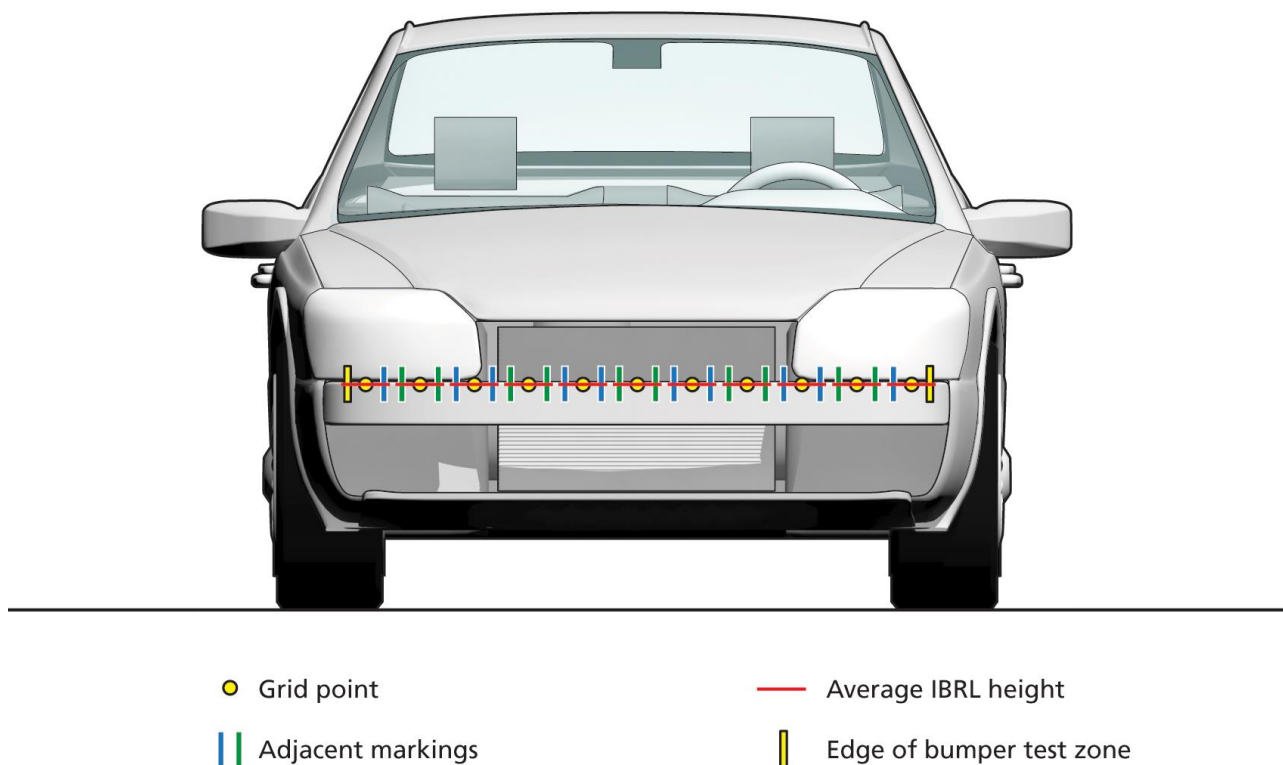
Figure 15: IBRL height at 100mm intervals
