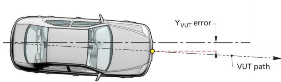
Figure 2: Lateral path error
