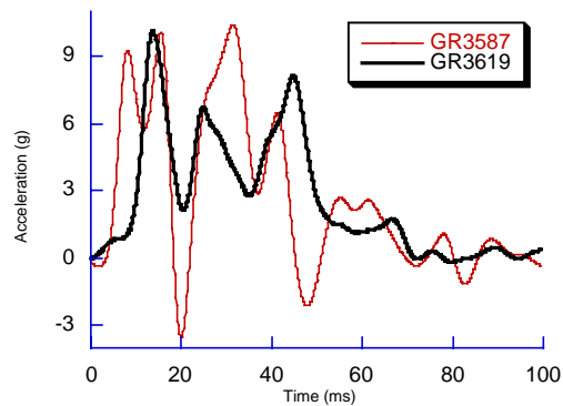
Figure A11. The acceleration pulse measured at the bottom of the B-pillar in the 40% overlap barrier test producing a delta-v of 9.0 km/h and 9.1 km/h.
