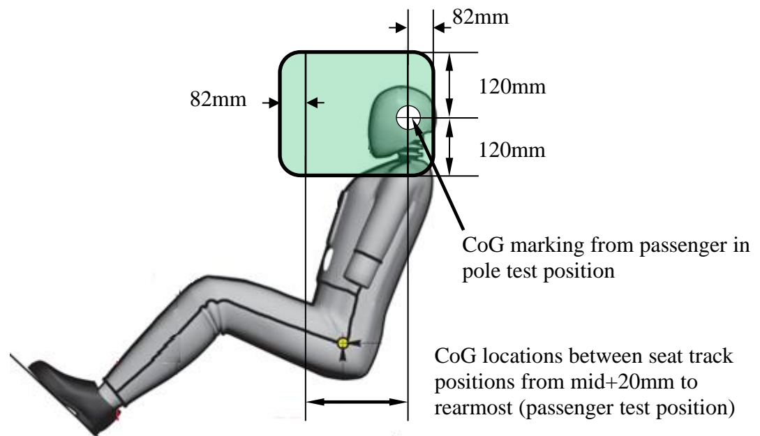
Figure 6: Protection zone
