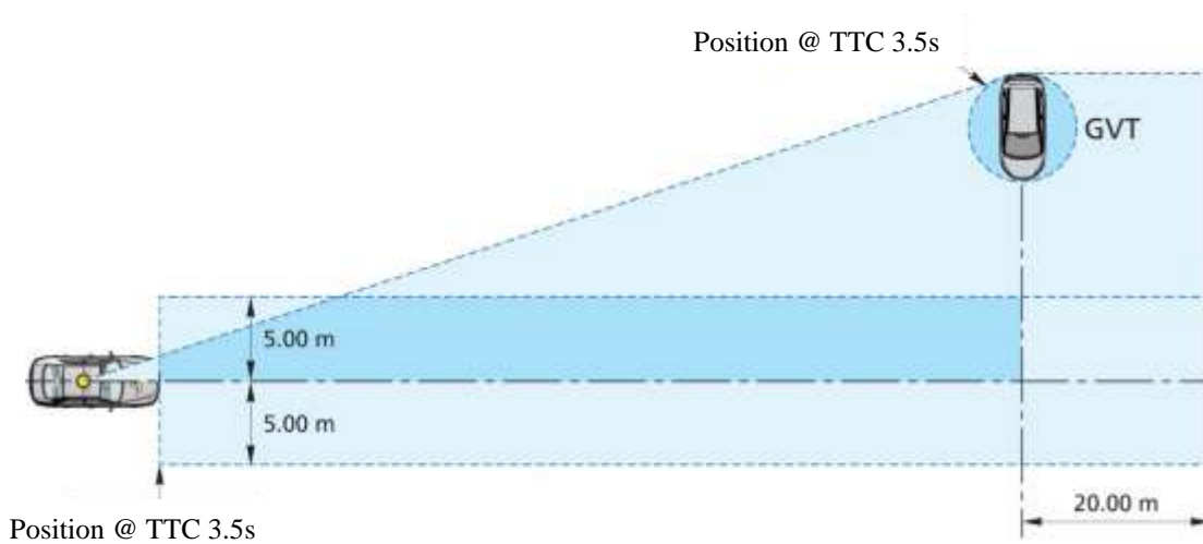
Figure 7-3: Free space requirements – CCC Farside Test
