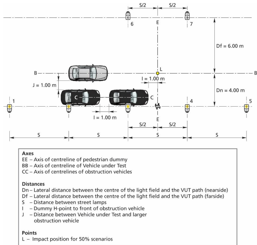
Figure B9: CPNCO Night-time setup
