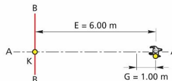
Figure 7-6 CPTA scenario – VUT left turn, pedestrian crossing from nearside
