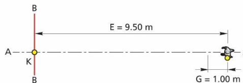
Figure 7-7 CPTA scenario – VUT right turn, pedestrian crossing from farside
