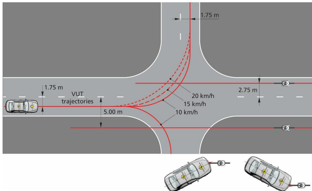
Figure 7-14: CBTA scenarios, Turning cycling Adult
