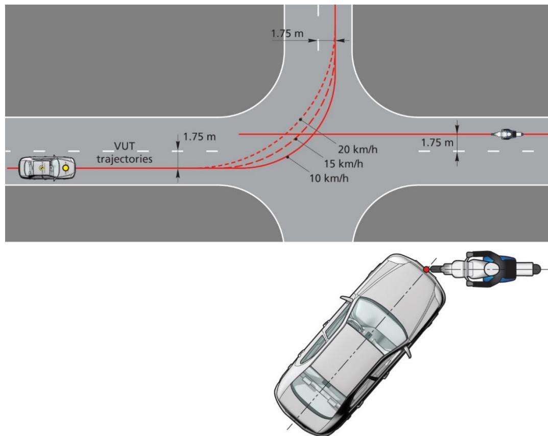
Figure 7-19: CMFtap scenario VUT and EMT paths
