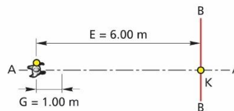
Figure 7-8 CPTA scenario – VUT right turn, pedestrian crossing from nearside
