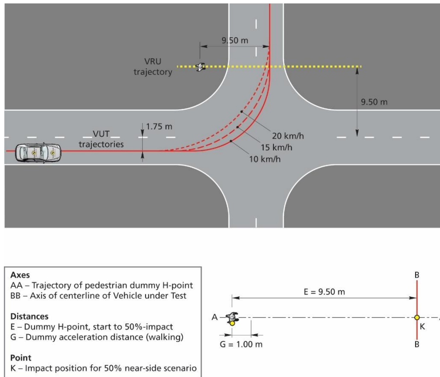
Figure 7-5: CPTA scenario – VUT left turn, pedestrian crossing from farside
