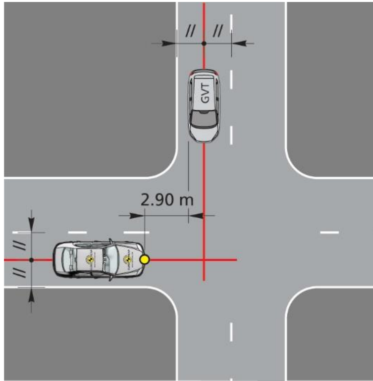
Figure 8-9 SCP start from stop setup
